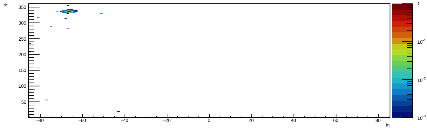
0.1 GeV Case: Full ECAL (Check for two dots side-by-side)
