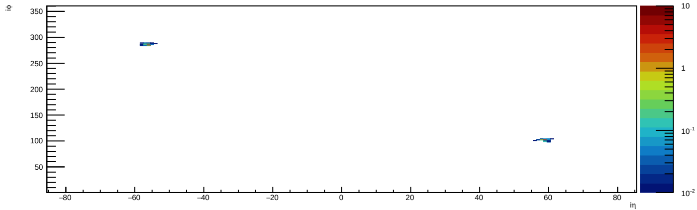
10 GeV Case: Full ECAL (Check for two dots at opposite iEta)
